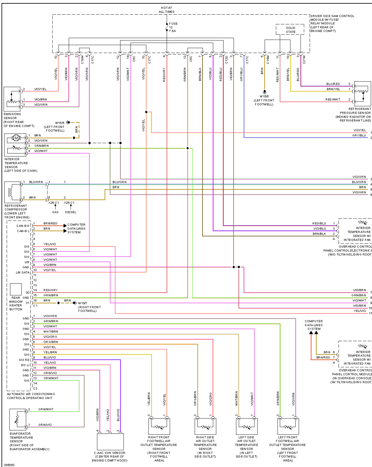
Fig. 5: Automatic A/C Circuit, Sedan W/ Thermotronic (1 of 3)
