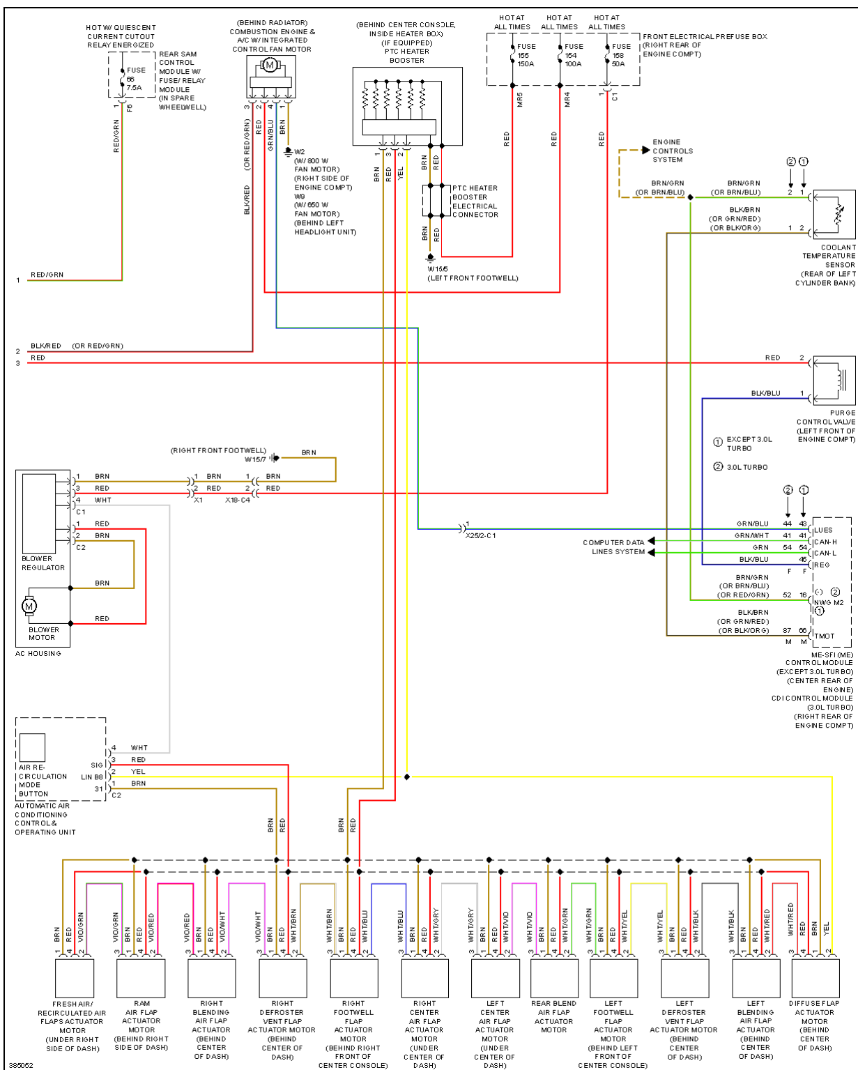
Fig. 7: Automatic A/C Circuit, Sedan W/ Thermotronic (3 of 3)
