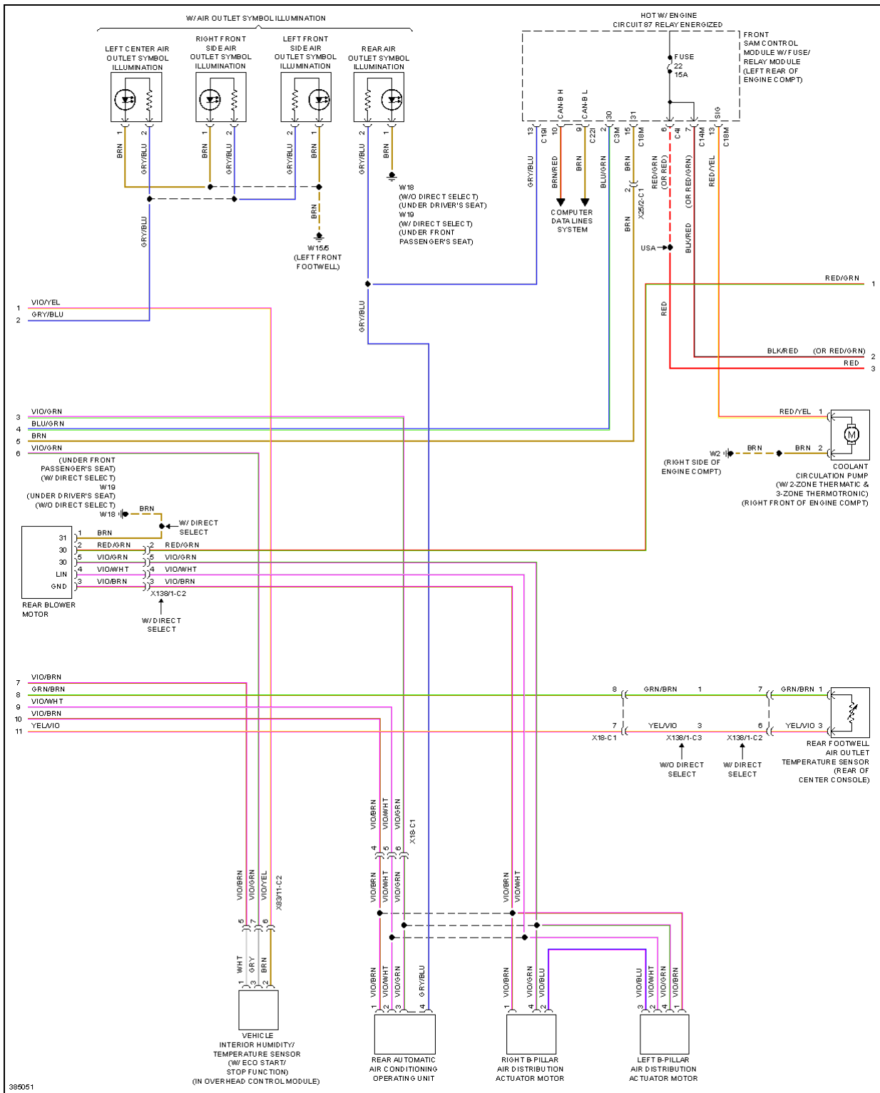
Fig. 6: Automatic A/C Circuit, Sedan W/ Thermotronic (2 of 3)
